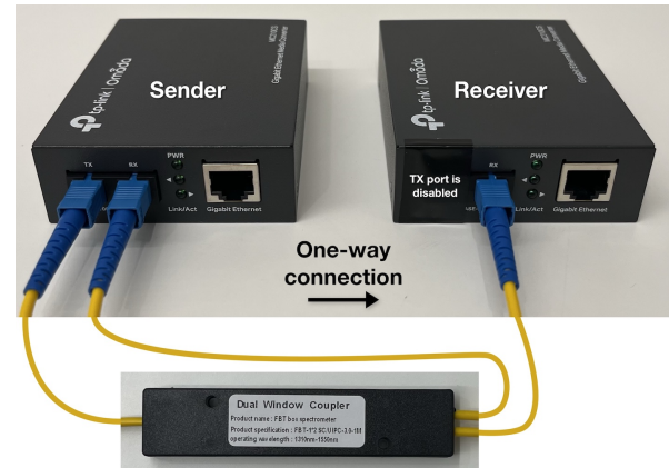
Figure 1: A data diode built with Ethernet fiber-optic media converters. The converter on the left sends data to the converter on the right. The converter on the right physically cannot transfer data in the reverse direction, since its transmit port is taped over.
