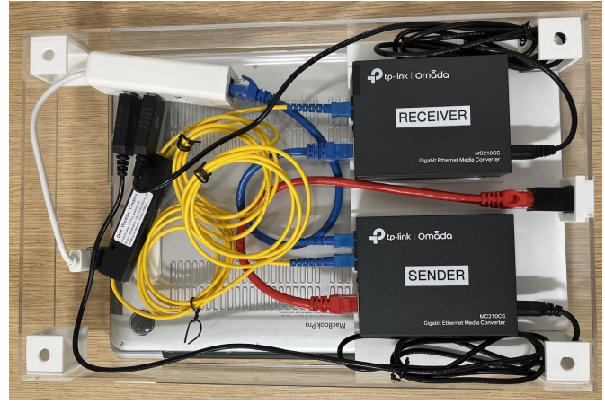
(b) The enclosure underneath the air-gapped laptop contains a data diode. The data diode consists of two Ethernet fiber-optic media converters, one of which has its transmit port taped over. This configuration physically enforces the direction of network traffic, preventing the laptop from sending data to the smartphone.
